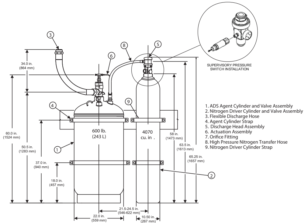
Figure 1. Single Cylinder Installation Dimensions, 600 lb. (243 L) Cylinder
