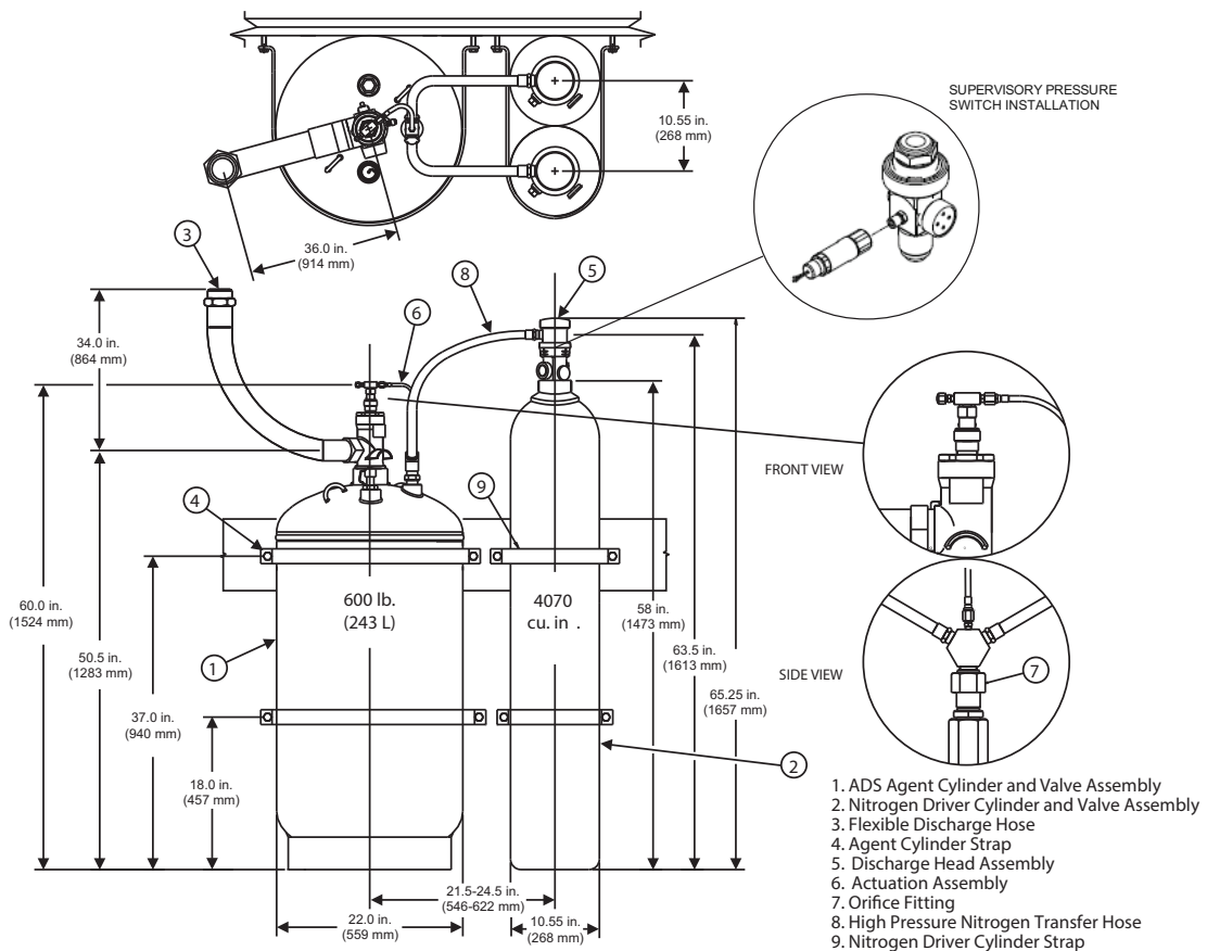
Figure 2. Dual Driver Installation, Vertical Mounting for 600 lb. (243 L) Systems
